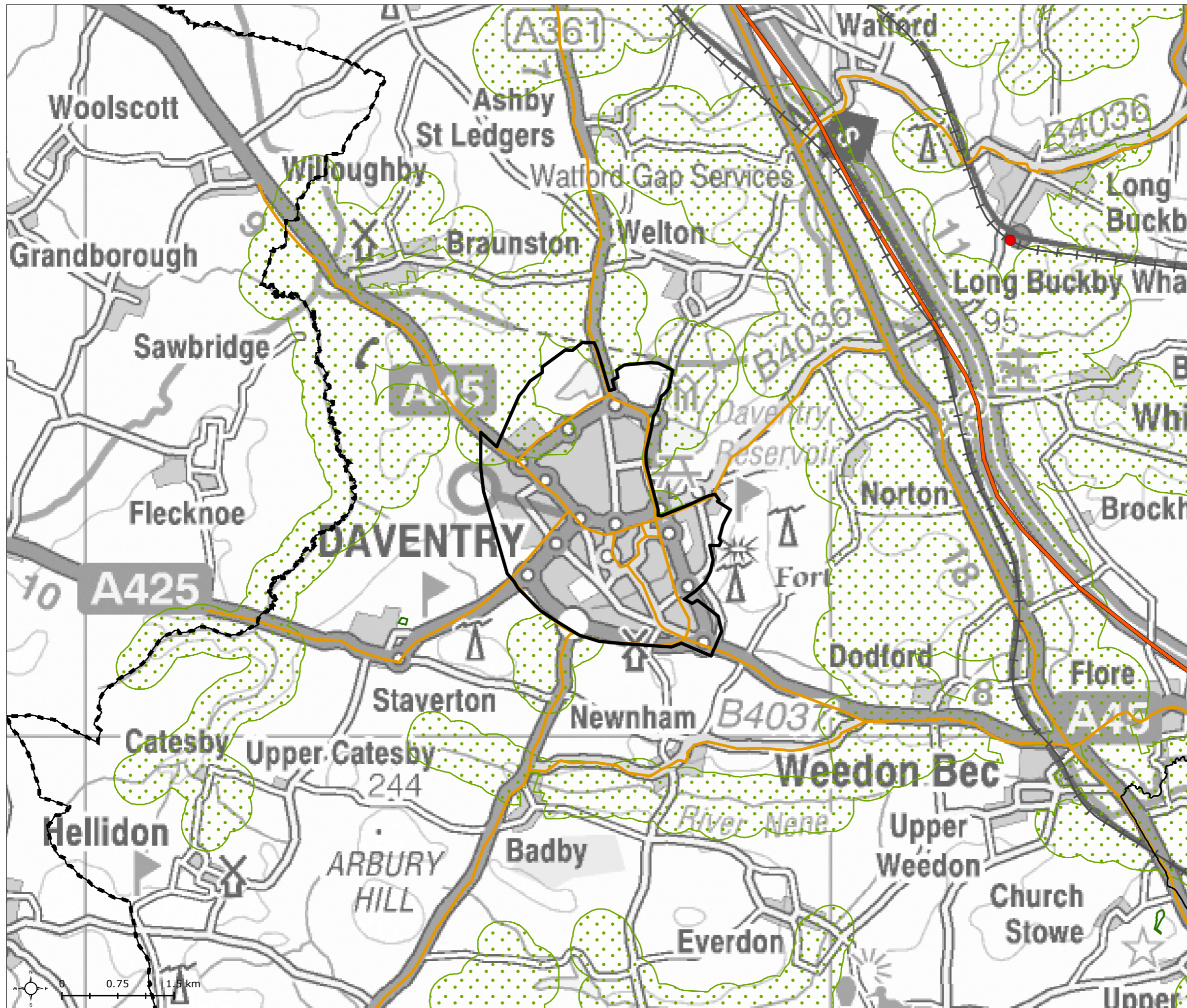
Figure: A6 Daventry - Geology and Minerals
